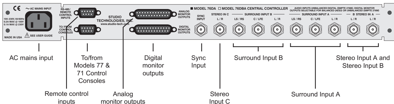
Figure 2. Model 76DA Central Controller Back Panel
